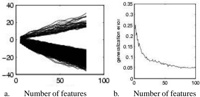
Figure 1: Stopping criteria for Adaboost training. a. Output of one expression classifier during Adaboost training. The response for each of the training examples is shown as a function of number features as the classifier grows. b. Generalization error as a function of the number of features chosen by Adaboost. Generalization error does not increase with 'overtraining'.
