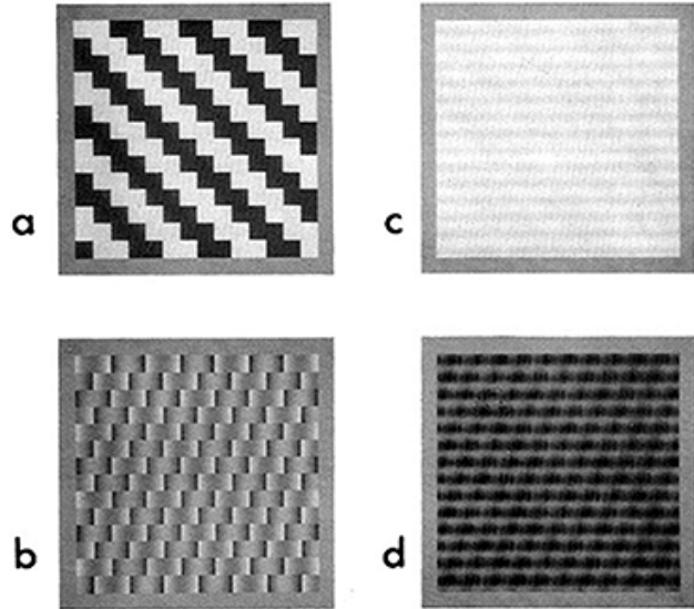
Fig. 17. a, An (x, t) plot of a square wave's motion. b, A (x, t) plot of a fluted square wave's motion. c, The response of a medium spatial-frequency opponent-motion channel when stimulated by the square wave. Rightward motion (bright) is signaled. d, The response of the same channel when stimulated by the fluted square wave. Leftward motion (dark) is signaled.
