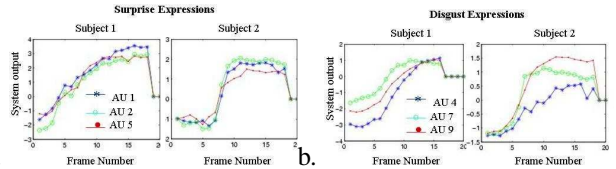
Figure 7: Automated FACS measurements for full image sequences. a. Surprise expression sequences from 2 subjects scored by the human coder as containing AU's 1,2 and 5. Curves show automated system output for AU's 1,2 and 5. b. Disgust expression sequences from 2 subjects scored by the human coder as containing AU's 4,7 and 9. Curves show automated system output for AU's 4,7 and 9.
